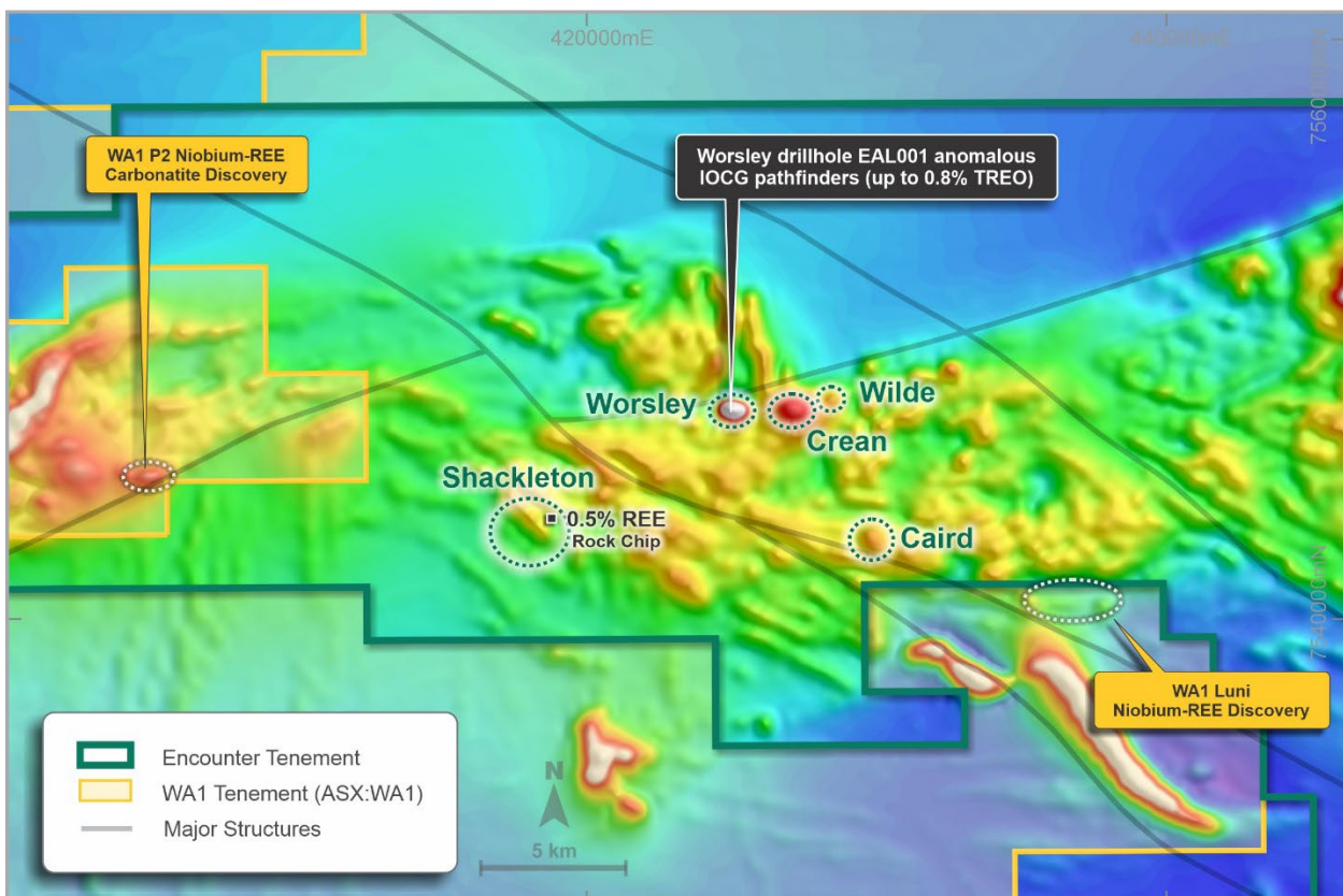
Figure 1 – Aileron Cu-REE project – Magnetics (TMI) 1,2,3,4
