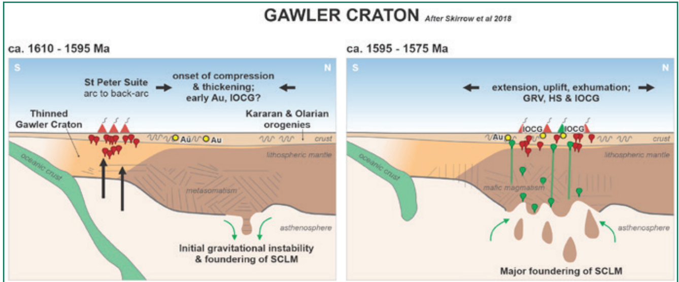
Figure 4 - IOCG Gawler Craton Schematic Model - modified from Skirrow et al 2018
